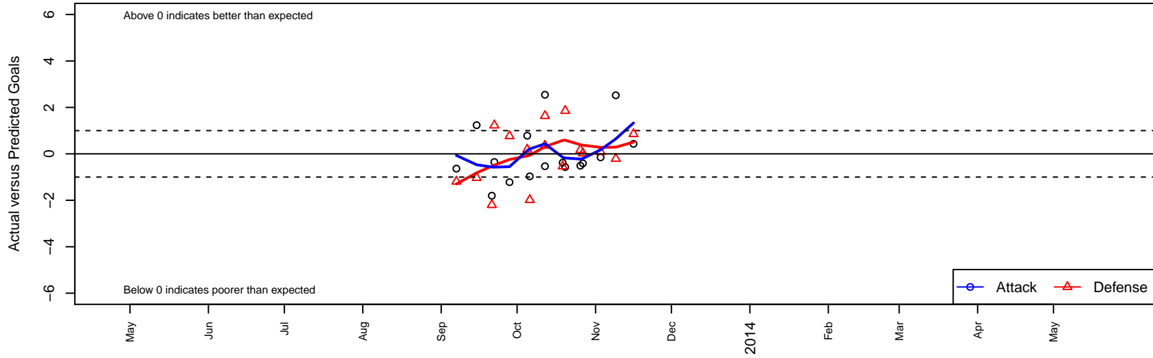
Westside Breakers White G00 Dots are actual minus expected GF (blue circles) and GA (red triangles). Blue line is smoothed change in attack strength. Red is smoothed change in defense strength.
